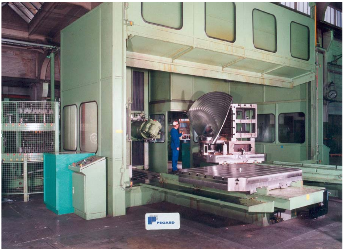
TAMPELLA FINLAND : 5 AXES MACHINING OF PROPELLERS BLADES
