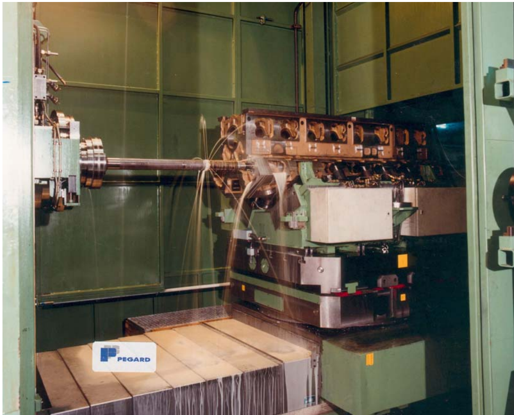
KCL INDIA : MACHINING OF THE CAMSHAFT BEARINGS
