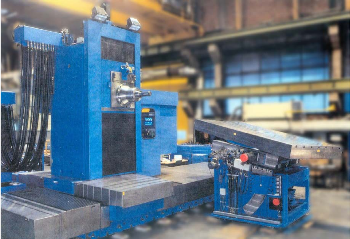
BOEING : PRECIVIT 2 WITH CNC TILTING-TABLE (360 000 ROTARY AXIS) WITH 5.7 KW POWER MAXIMUM LOAD :10 000 kg
