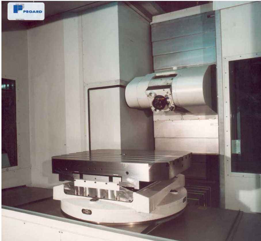
MBB (DEUTSCHE AIRBUS) : FLEXIVIT WITH ELECTRO-SPINDLE
